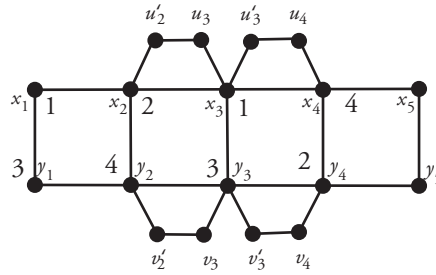
Figure 5. A partial coloring of OG_5^- .
