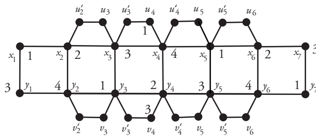
Figure 6. A partial coloring of OG_7^- .
