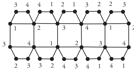
Figure 3. A star coloring of OG_6 with 4 colors.
