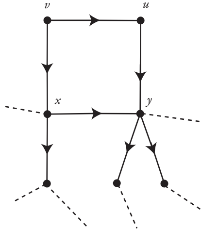
Figure 1. Extending the in-coloring to u and v .
