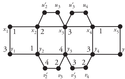
Figure 4. A partial coloring of OG_5^- .
