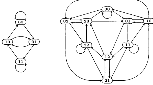
Figure 2.1. The graphs B_2^{(2)} and B_2^{(3)}
