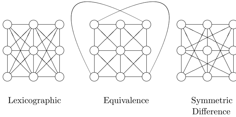
Figure 1b. P_3 \bullet P_3 , P_3 \oplus P_3 & P_3 \nabla P_3 .
