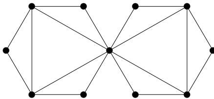
Figure 1. A graph with leafage 4 but no asteroidal 4-set
