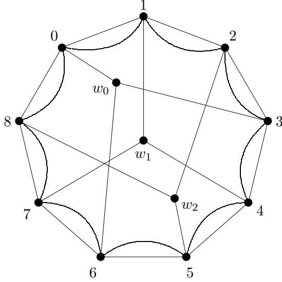
Figure 1. Multigraph M_1
