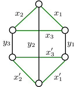
Figure 10. Marking the numbers of the crossings for the graph P(3, 1) .
