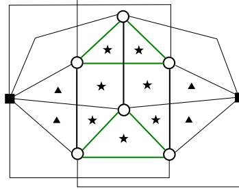
Figure 13. The subdrawings of W in the drawing of P(3, 1) + nK_1 .
