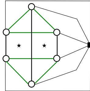
Figure 11. The subdrawings of F in the drawing of P(3, 1) + nK_1 .
