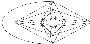
Figure 1. The drawing of the graph P(3, 1) + nK_1 .
