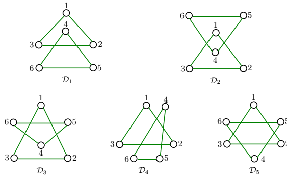
Figure 3. The possible subdrawings of C'_3 \cup C''_3 , if cr_D(C'_3, C''_3) \neq 0 .
