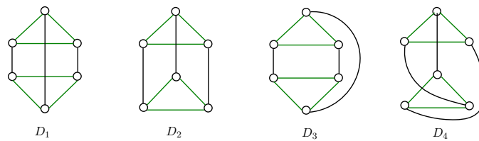
Figure 9. The possible subdrawings of P(3, 1) in the optimal drawing P(3, 1) + nK_1 .
