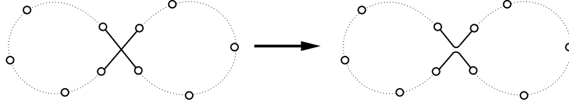
Figure 15. Removing the self-crossings on the edges C_n^* .
