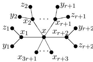
Figure 1. Family \mathcal{F} .
