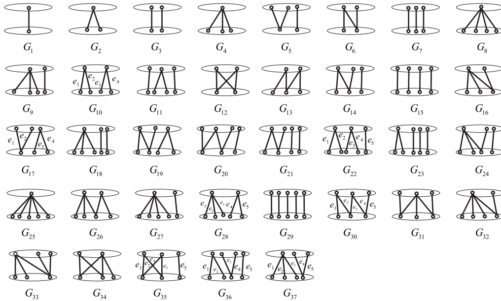
Figure 1. All graphs obtained from K_{p,p} by deleting five or fewer edges drawn.
