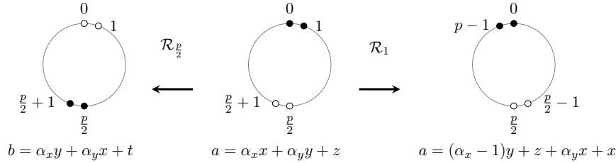
Figure 16. Rotations of the colouring c of a Type 2 cycle with c(\frac{p}{2}) = 0 = c(\frac{p}{2} + 1) , and their corresponding weighted sums of black vertices.
