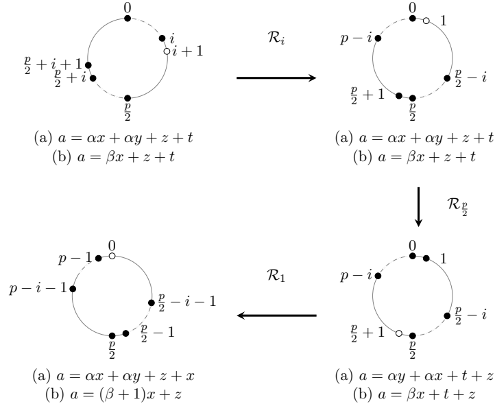
Figure 13. Rotations of the colouring c of a Type 2 cycle C_p with c(\frac{p}{2} + i + 1) = 1 , and their corresponding weighted sums of black vertices which are not all equal, where the line (a) corresponds to the case x \neq y and the line (b) to the case x = y .
