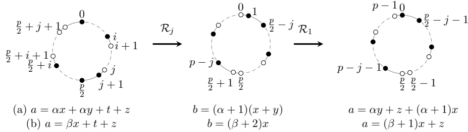
Figure 15. Rotations of the colouring c of a Type 2 cycle with c(j + 1) \neq c(\frac{p}{2} + j + 1) = 0 , and their corresponding weighted sums of black vertices which are not all equal, where the line (a) corresponds to the case x \neq y and the line (b) to the case x = y .
