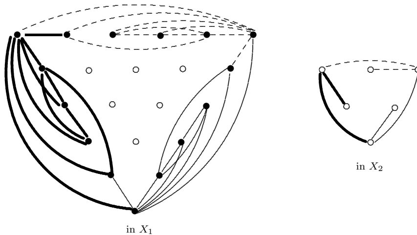
Figure 10. Edges in the two triangular sets X_1 and X_2 for G_8 .
