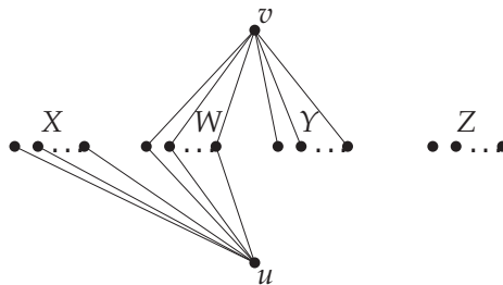
Figure 2. Partition of R depending on whether or not w \in R is adjacent to u or v .
