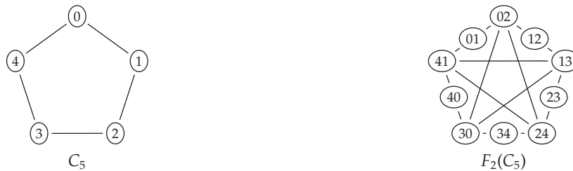
Figure 1. The cycle graph C_5 and its token graph F_2(C_5) .
