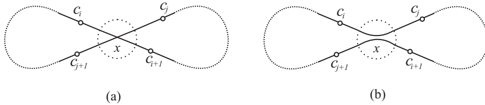
Figure 1. Elimination of a crossing in C_n .
