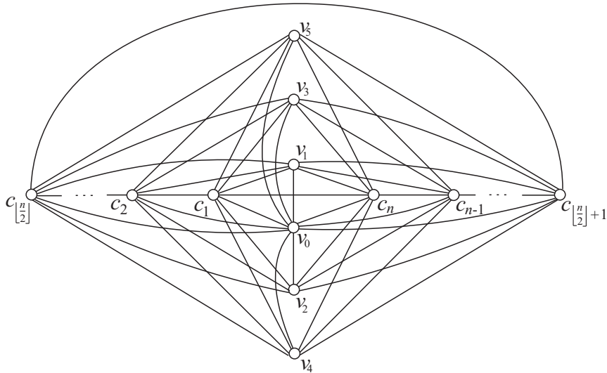
Figure 2. The drawing of the graph S_5 + C_n .
