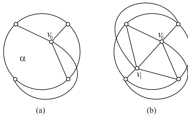
Figure 3. The subdrawings of C_4 \cup T^{v_0} and C_4 \cup T^{v_0} \cup T^{v_1} \cup \{v_0, v_1\} .
