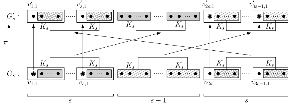
Figure 1. The graph \pi((3s - 1)K_s) . The set of s(s - 1) vertices in gray (resp. lined, squared) rectangles below map to the set of s(s - 1) vertices in gray (resp. lined, squared) rectangles above. The set of encircled vertices is a distance 2-dominating set.
