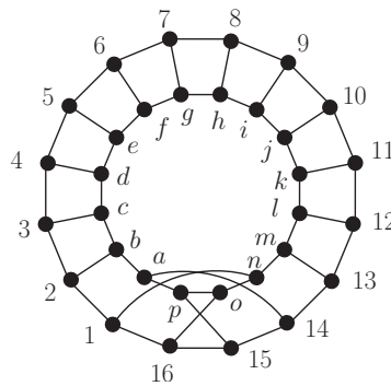
Figure 6. The graph \pi C_{16} .
