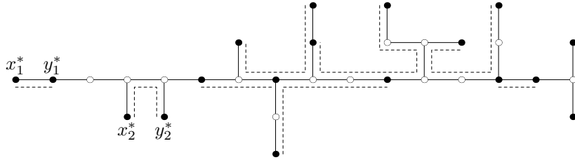
Figure 3. A minimal subtree S .
