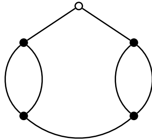
Figure 5. The gadget G' used for the case q = 5 .
