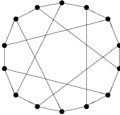
Figure 1. Heawood graph.
