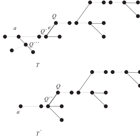
Figure 9. T and T' UV -model for Lemma 4.
