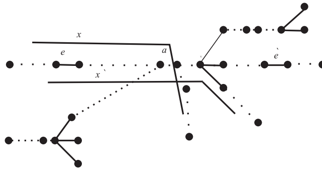
Figure 18. T UV-model; lab(e) \not\subseteq lab(e') , lab(e') \not\subseteq lab(e) and lab(e) \cap lab(e') = \emptyset .
