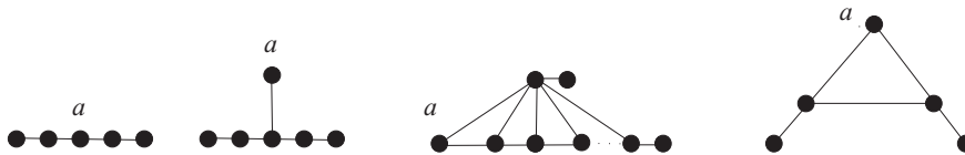
Figure 3. Gimbel’s graphs.
