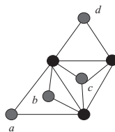
Figure 2. a, b, d are end vertices, c is not an end vertex.
