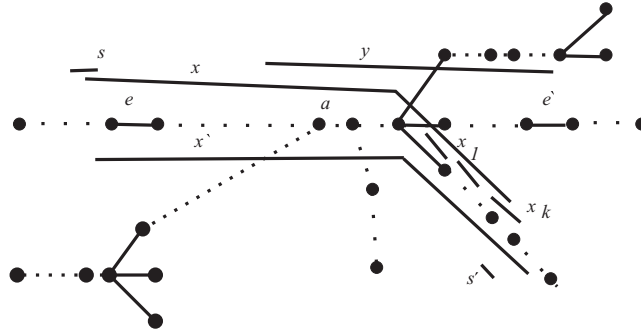
Figure 22. T UV-model; lab(e) \not\subseteq lab(e') , lab(e') \not\subseteq lab(e) and lab(e) \cap lab(e') = \emptyset .
