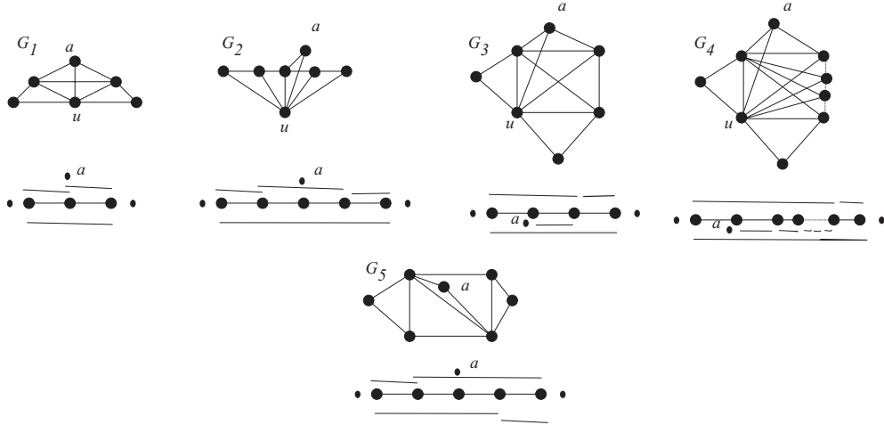
Figure 5. Graphs and its unique UV -models.
