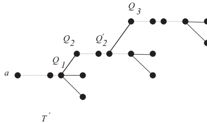
Figure 8. T' UV -model for Lemma 3. ■
