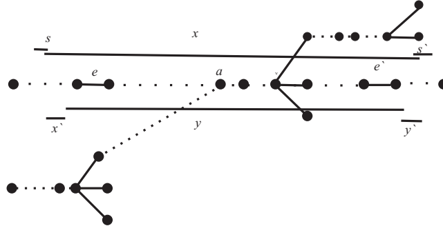
Figure 11. T UV-model, lab(e) = lab(e') .
