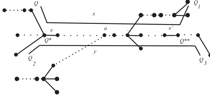
Figure 13. T UV-model, lab(e) = lab(e') .
