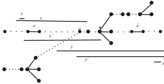
Figure 17. T UV-model; lab(e) \not\subseteq lab(e') , lab(e') \not\subseteq lab(e) and lab(e) \cap lab(e') = \emptyset .
