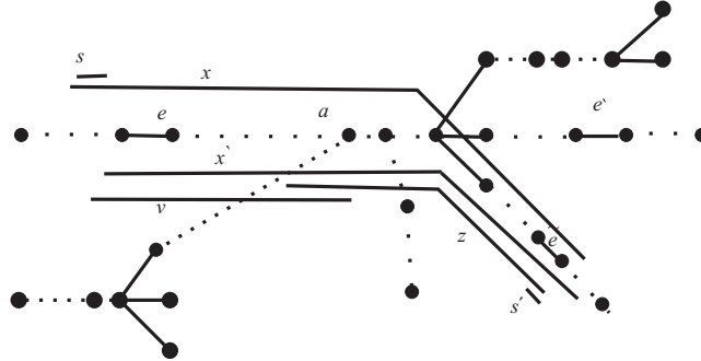
Figure 21. T UV-model; lab(e) \not\subseteq lab(e') , lab(e') \not\subseteq lab(e) and lab(e) \cap lab(e') = \emptyset .
