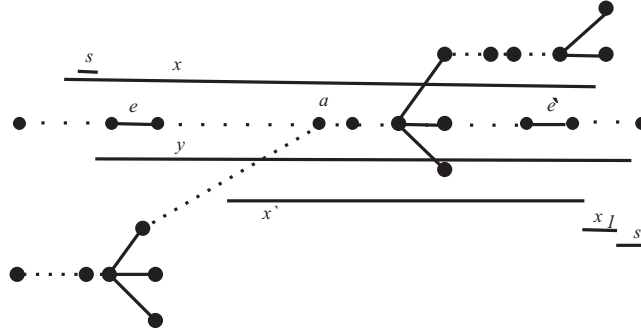
Figure 14. T UV-model, lab(e) \subset lab(e') and lab(e') \not\subseteq lab(e) .
