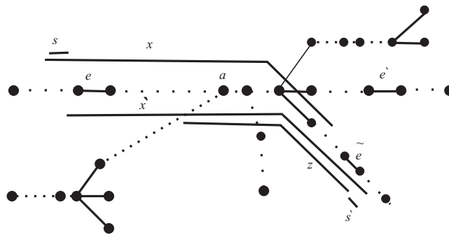
Figure 19. T UV-model; lab(e) \not\subseteq lab(e') , lab(e') \not\subseteq lab(e) and lab(e) \cap lab(e') = \emptyset .
