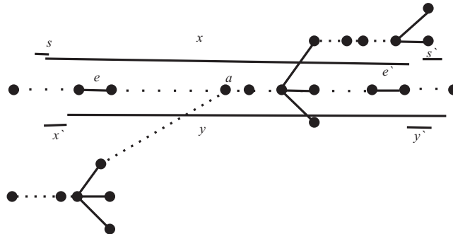
Figure 12. T UV-model, lab(e) = lab(e') .
