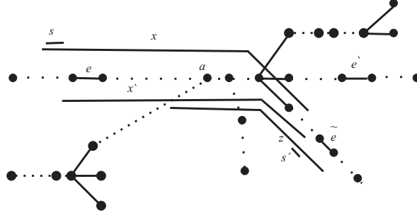
Figure 20. T UV-model; lab(e) \not\subseteq lab(e') , lab(e') \not\subseteq lab(e) and lab(e) \cap lab(e') = \emptyset .
