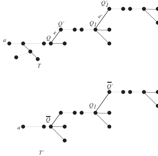
Figure 10. T and T' UV -model for Lemma 5.
