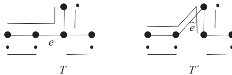
Figure 7. Equivalent edges.
