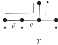
Figure 6. Twin edges.
