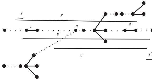
Figure 15. T UV-model, lab(e) \subset lab(e') and lab(e') \not\subseteq lab(e) .
