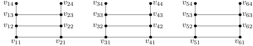
Figure 2. The graph T_6^+ .
