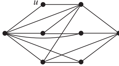
Figure 1. \gamma_m^\infty(G) = \alpha(G) = 3 .
