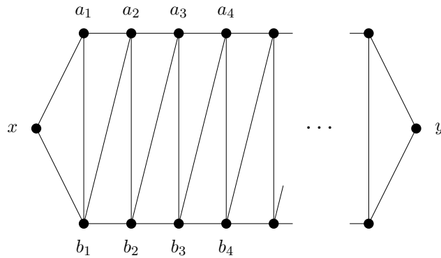
Figure 2. The structure of G , with relabelled vertices.
