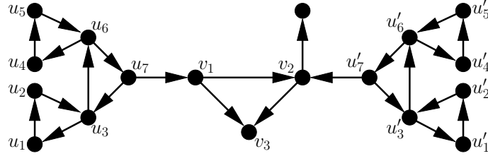
Figure 1. The forbidding gadget \overrightarrow{F}_{3,4} .
