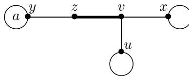
Figure 7. Configuration for Lemma 3.3.
