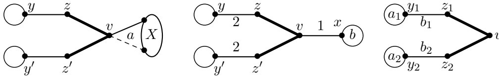
Figure 5. Case B for Lemma 2.9
