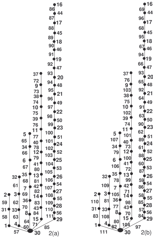
Figure 2. (a) Super (88,2)-EAT labeling of the subdivided star T(3,4,7,14,27) . (b) Super (115,1)-EAT labeling of the subdivided star T(3,4,7,14,27) .
