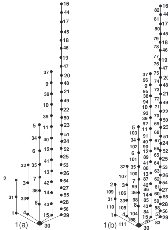
Figure 1. (a) (31,1)-EAV labeling of the subdivided star T(3,4,7,14,27) . (b) Super (142,0)-EAT labeling of the subdivided star T(3,4,7,14,27) .
