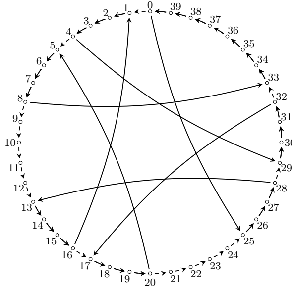
Figure 2. Exceptional case considered in Lemma 9: d = 8 .
