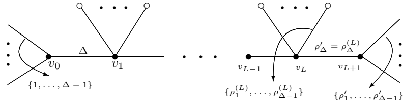
Figure 3. Shift of the precoloring from v_{L+1} to v_L in Proposition 8.
