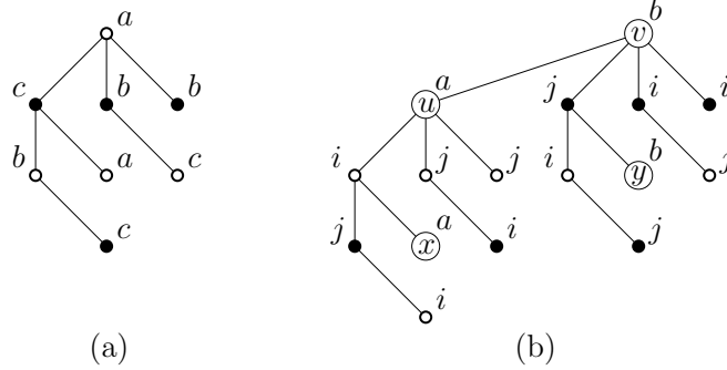
Figure 1. (a). The coloring g_{(a,b,c)} of B_3 , (b). the coloring of two subtrees B_3(u) and B_3(v) with uv \in E(B_{3k}) .
