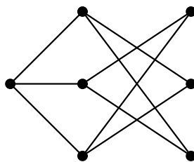
Figure 1. The smallest non- b -continuous graph.
