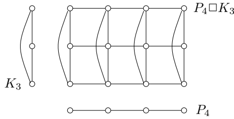
Figure 3. An illustration of Theorem 2.3. Here \alpha(K_3 \square P_4) = 2r(K_3)r(P_4) = 4 , and P_4 is a 2r -path, and \alpha_2(K_3) = 2r(K_3) = 2 .
