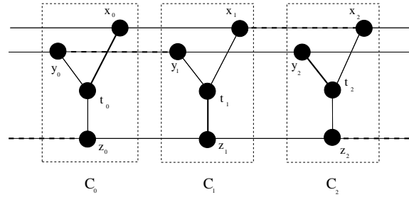
Figure 5. Strong matchings M_B (bold edges) and M_R (dashed edges).
