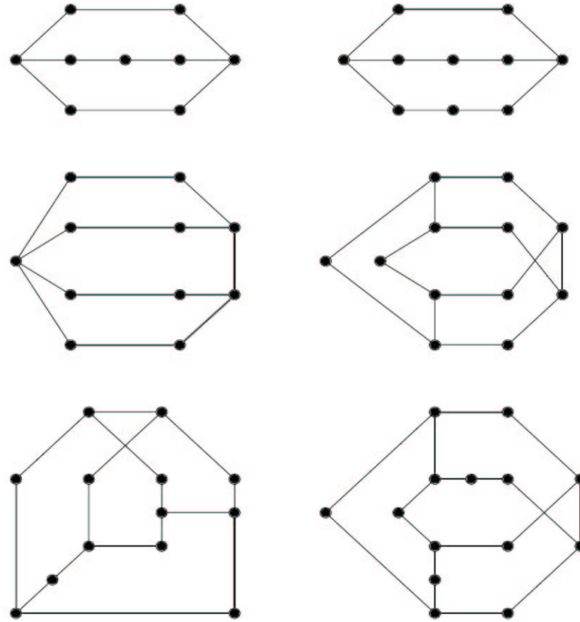
Figure 1. Graphs likely to minimize \lambda_1 + \bar{l} for n = 9, \dots, 14 .
