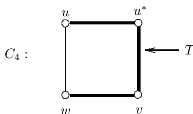
Figure 4. The 4-cycle C_4 and a spanning tree T in C_4 .
