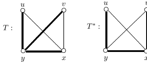
Figure 3. The converse of Observation 2.1 is false.
