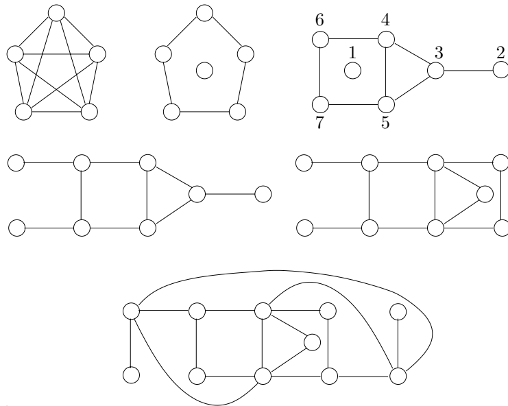
Figure 2. The exceptional critically non-bipartite graphs.
