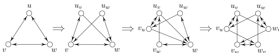
Figure 2. Elementary in-splittings that result in the line digraph.
