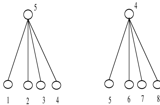
Figure 5. 1-segregated and 4-segregated star.
