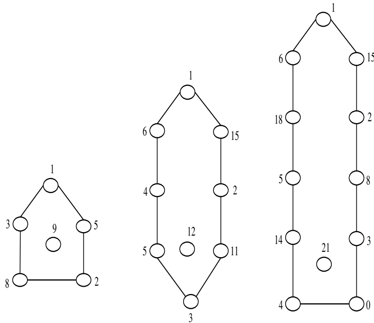
Figure 4. Sequentially additive cycles with one isolated vertex.
