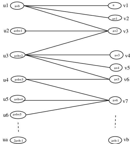
Figure 1. a -sequentially labeling of C_{a,b} .
