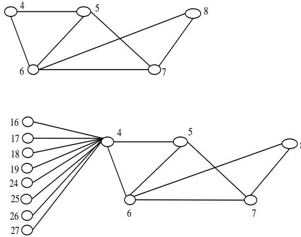
Figure 2. Illustration of Lemma 2.1.
