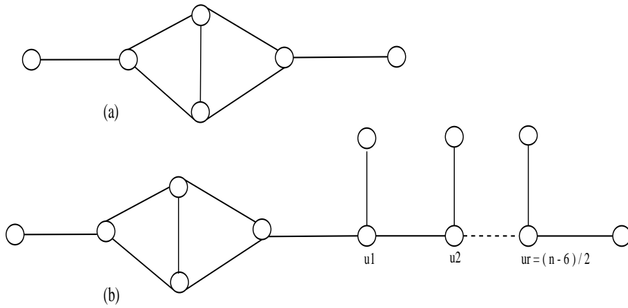
Figure 3. Odd-degree graphs.
