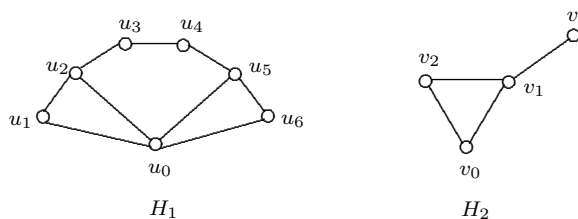
Figure 5. The graphs H_1 and H_2 in Case 2.
