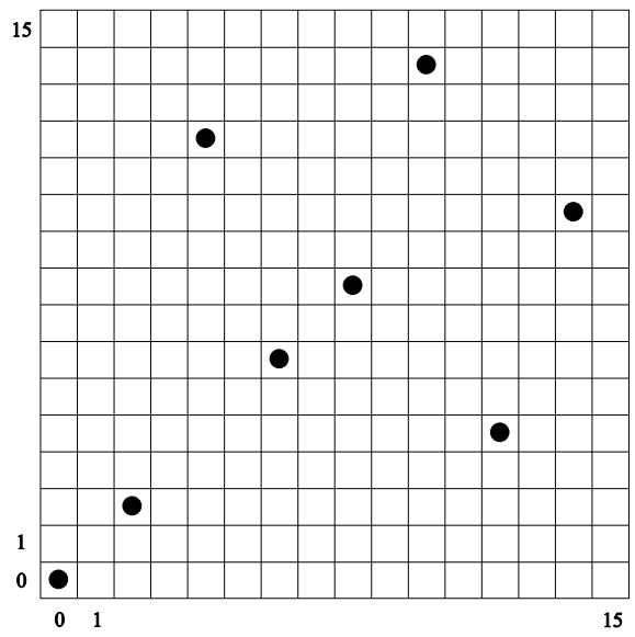
Figure 2. A dominating set of Q_{16}^t
