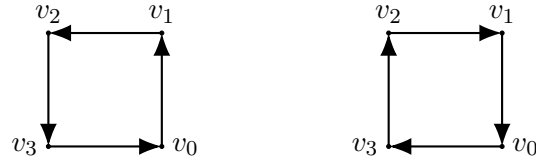
Figure 7. A packing of k = 2 copies of \vec{C}_4 .
