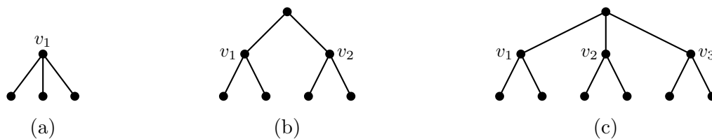
Figure 1. The three trees in the family \mathcal{T}_3 .
