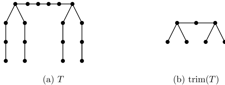
Figure 2. A tree T and its trimmed tree \text{trim}(T) .
