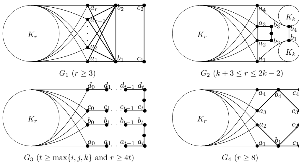
Figure 6. Some claw-o-heavy graphs.
