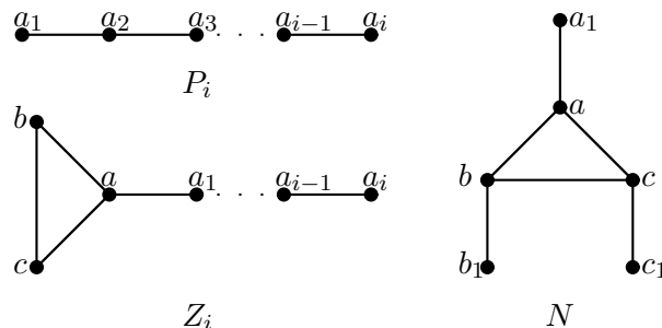
Figure 5. Graphs P_i , Z_i and N .
