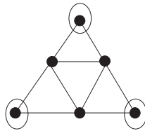
Figure 2. 3-sun containing an asteroidal triple.
