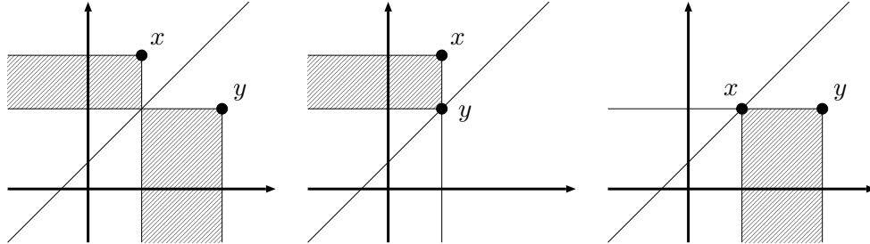
Figure 1. Pictures for Proof of Theorem 2.1.
