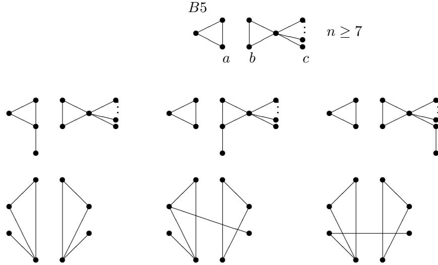
Figure 10. Cyclical embedding of graphs obtained from B5
