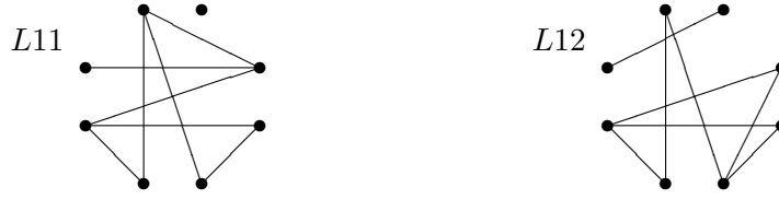
Figure 17. Cyclical embeddings of the graphs L11, L12
