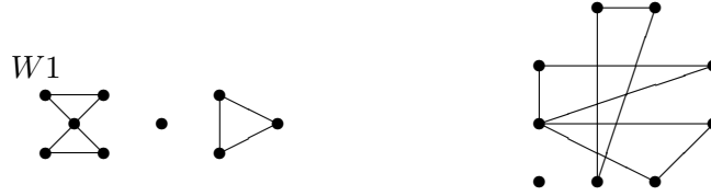
Figure 19. Graph W1 and its cyclical embedding
