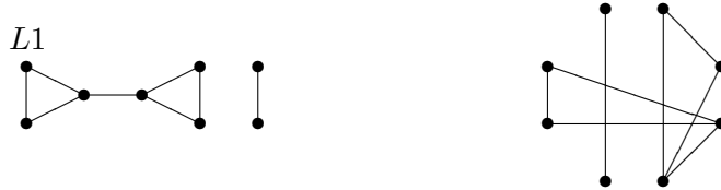
Figure 12. Graph L1 and its cyclical embedding
