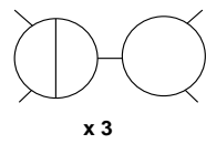
Figure 3. Dürer polyhedra on v = 10 + 2k vertices, ( k = 0, 1, 2, 3, 4 ), shown as bridges of the terminator circuit C(D^0) , each labelled with a multiplicity factor i.e., the number of non-isomorphic polyhedra derived by setting the given bridge in C .
