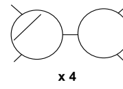
Figure 3. Dürer polyhedra on v = 10 + 2k vertices, ( k = 0, 1, 2, 3, 4 ), shown as bridges of the terminator circuit C(D^0) , each labelled with a multiplicity factor i.e., the number of non-isomorphic polyhedra derived by setting the given bridge in C .
