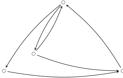
Figure 2. Digraph of type c . from Lemma 8.
