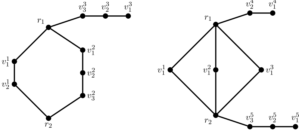
Figure 2. The partial balloons B(2, 3, \bar{3}) and B(1, 1, 1, \bar{2}, 3) .
