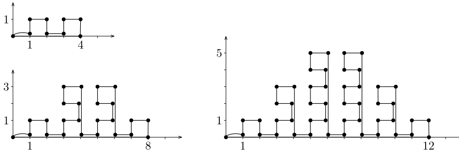
Figure 3. Grid diagrams for n = 9, 25, 49 .
