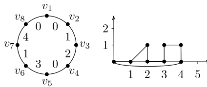
Figure 1. A detectable labeling of C_8 and the corresponding diagram.
