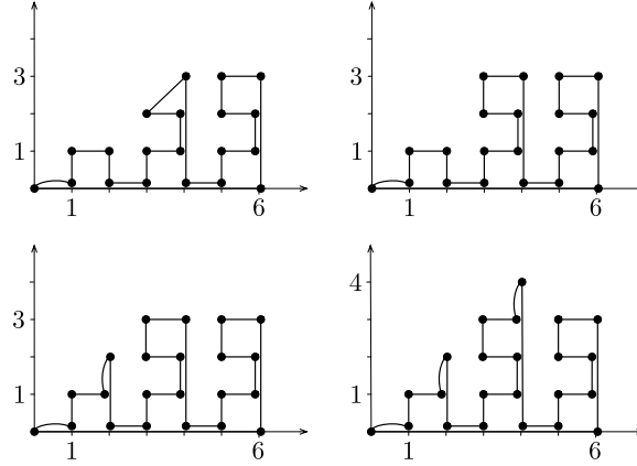
Figure 4. Grid diagrams for 20 \leq n \leq 23 .
